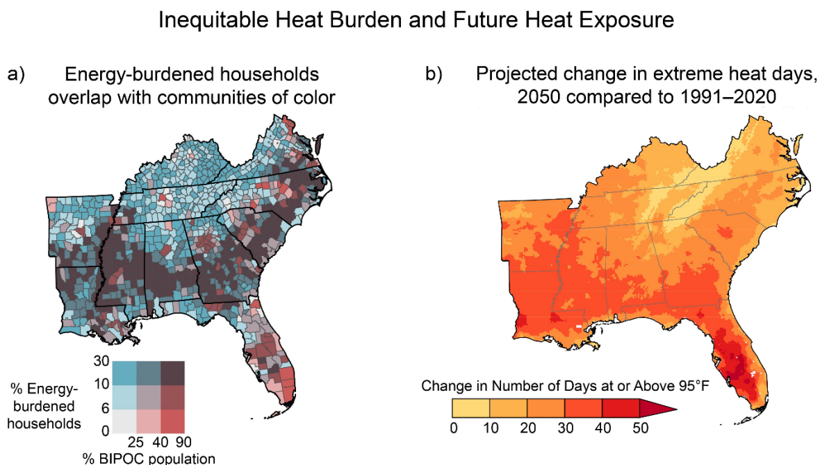
Figure 4.15 - Projected Change in Number of Days Over 95°F
